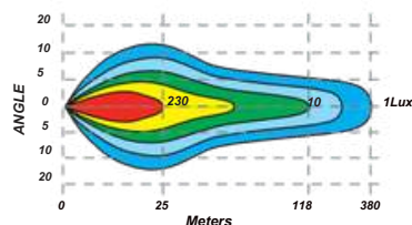
EURO BEAM
